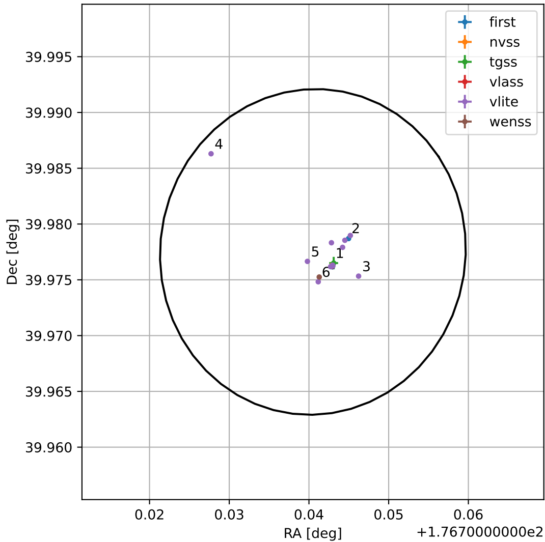
4FGL J1146.9+3958
