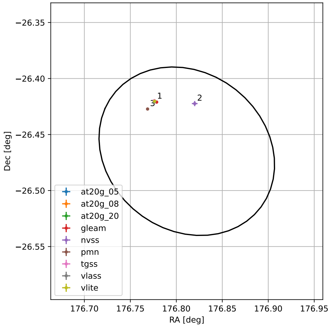
4FGL J1147.2-2627
