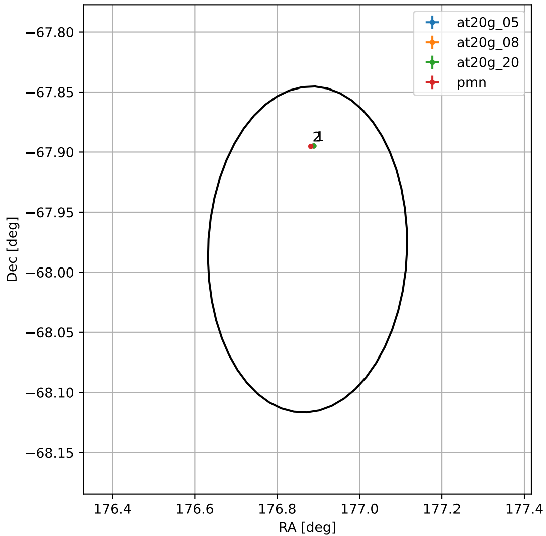
4FGL J1147.4-6758
