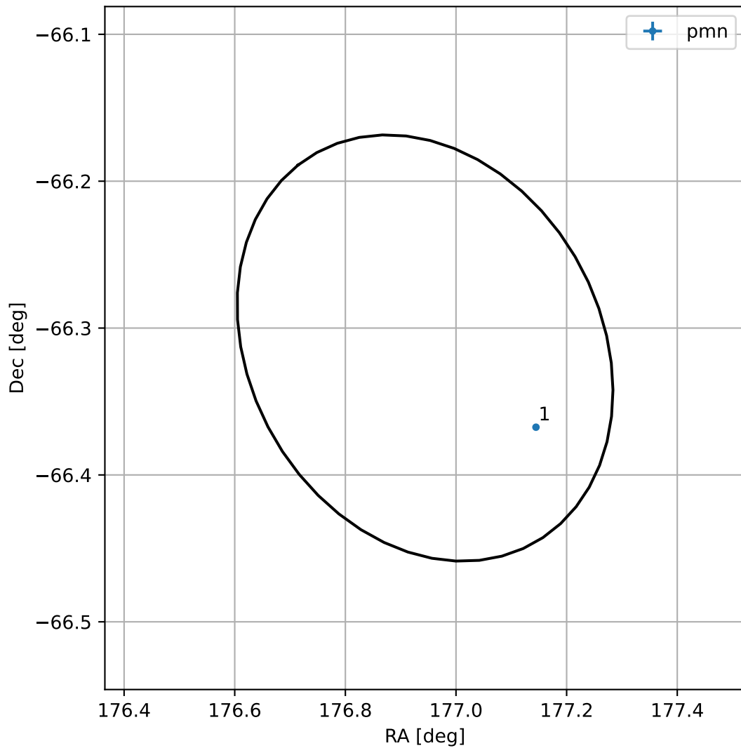
4FGL J1147.7-6618
