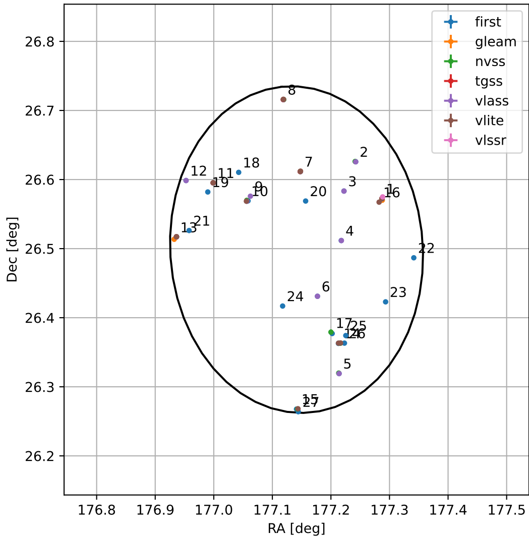
4FGL J1148.5+2629
