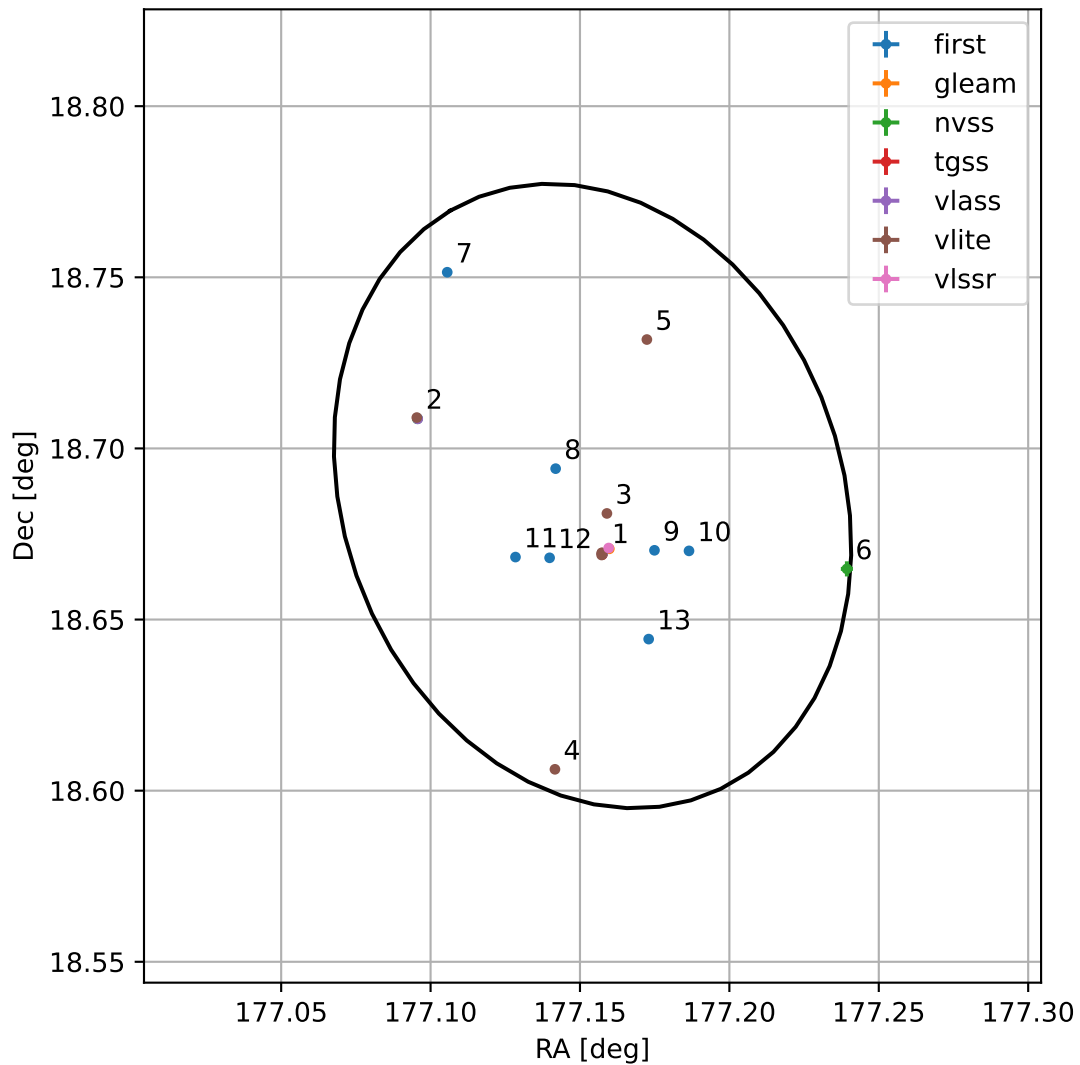
4FGL J1148.6+1841
