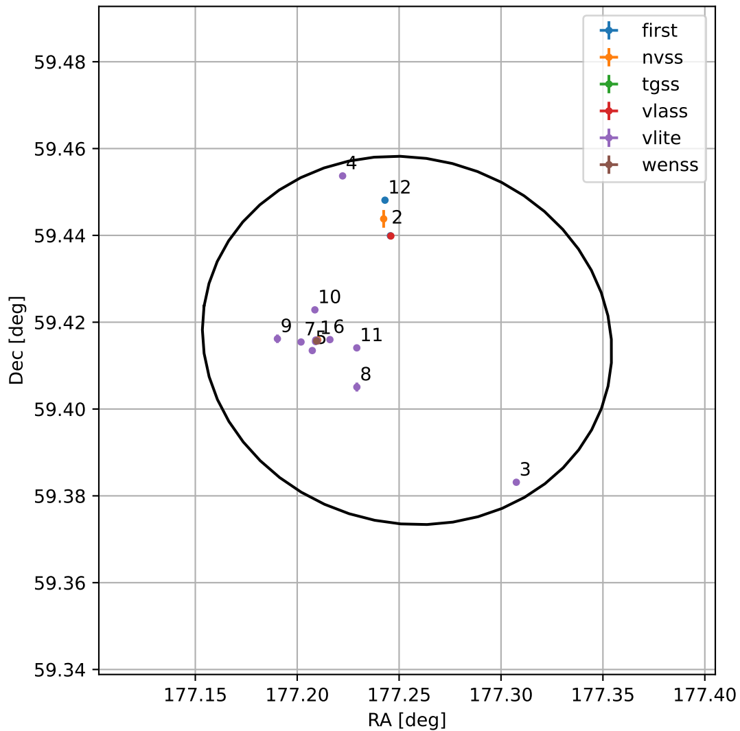
4FGL J1149.0+5924
