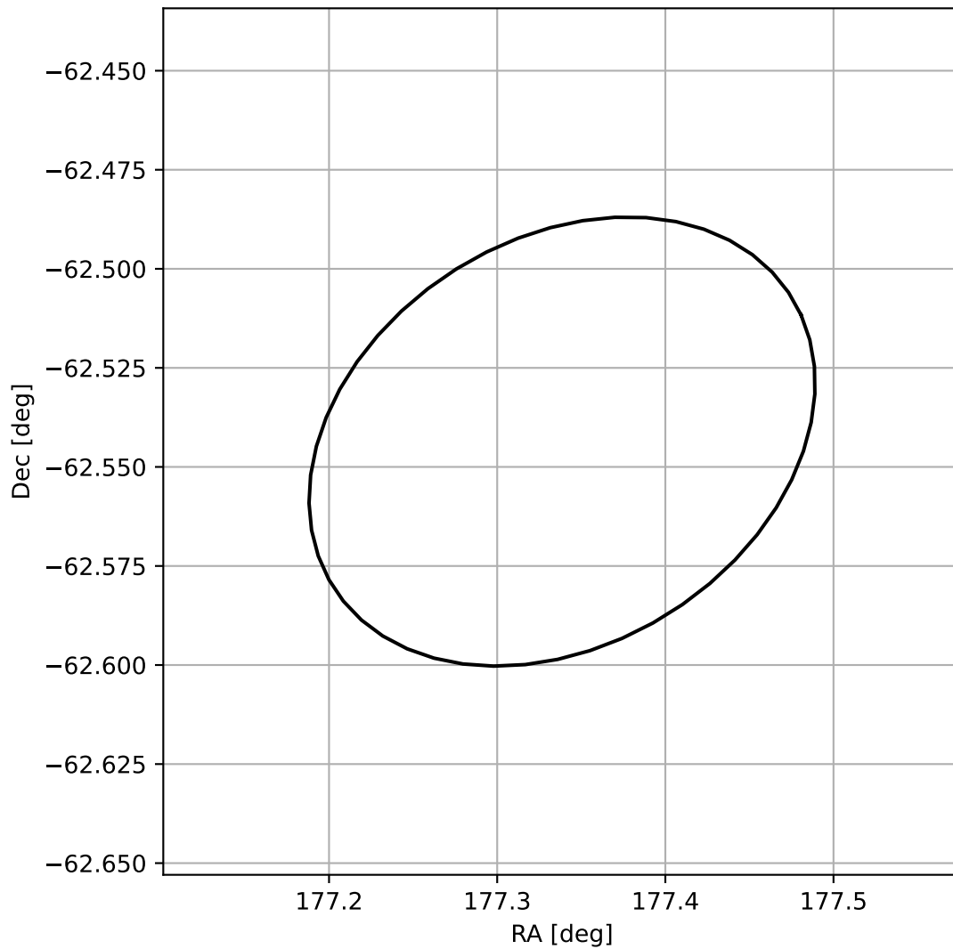
4FGL J1149.3-6232
