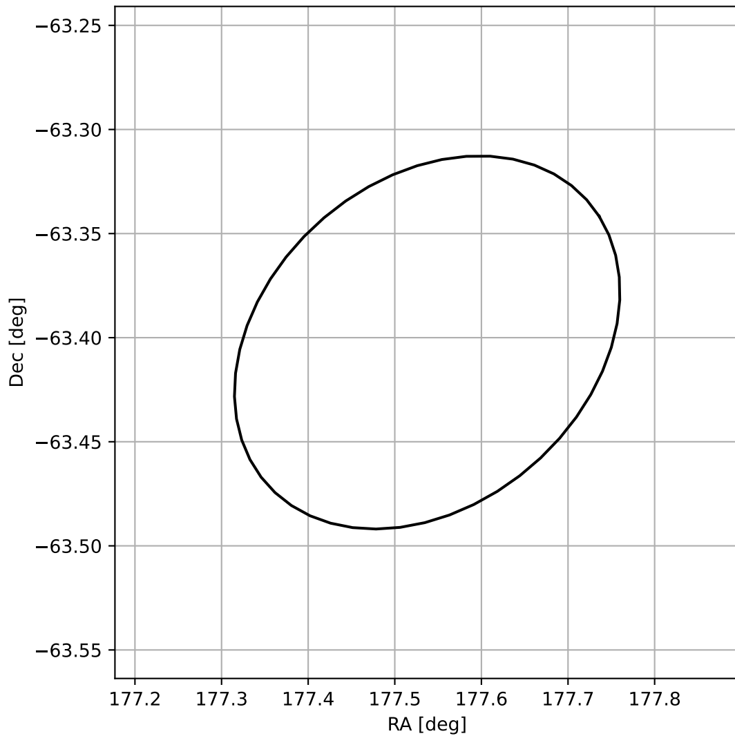
4FGL J1150.1-6324
