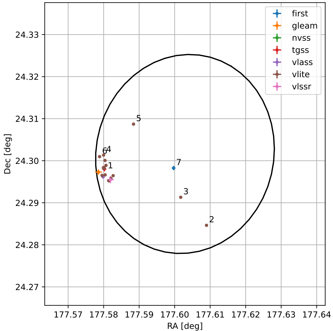
4FGL J1150.4+2418
