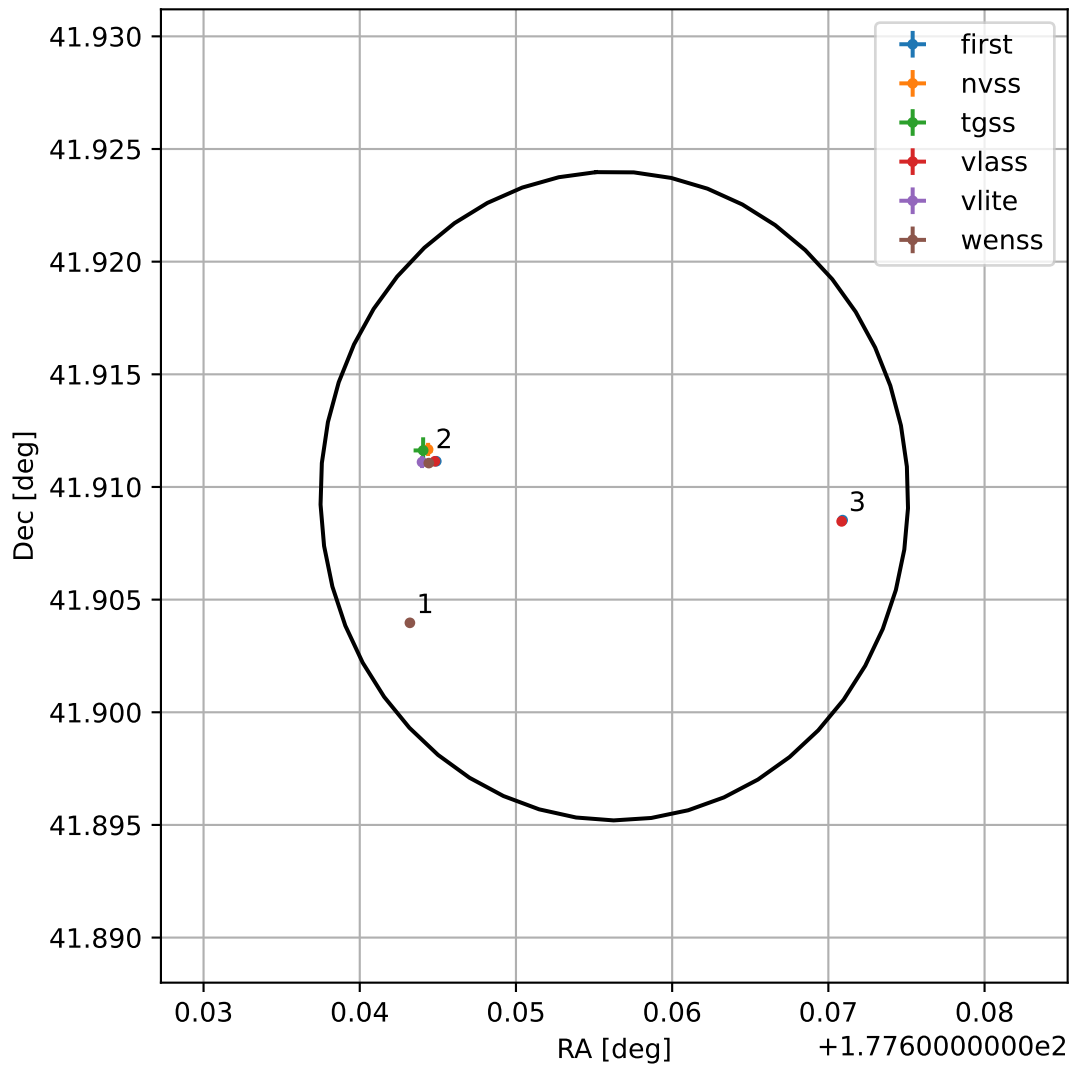
4FGL J1150.6+4154
