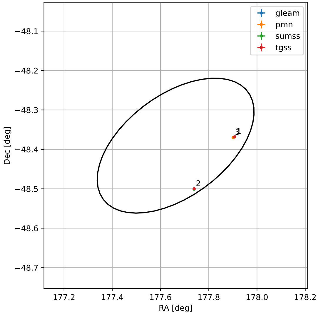
4FGL J1150.6-4823
