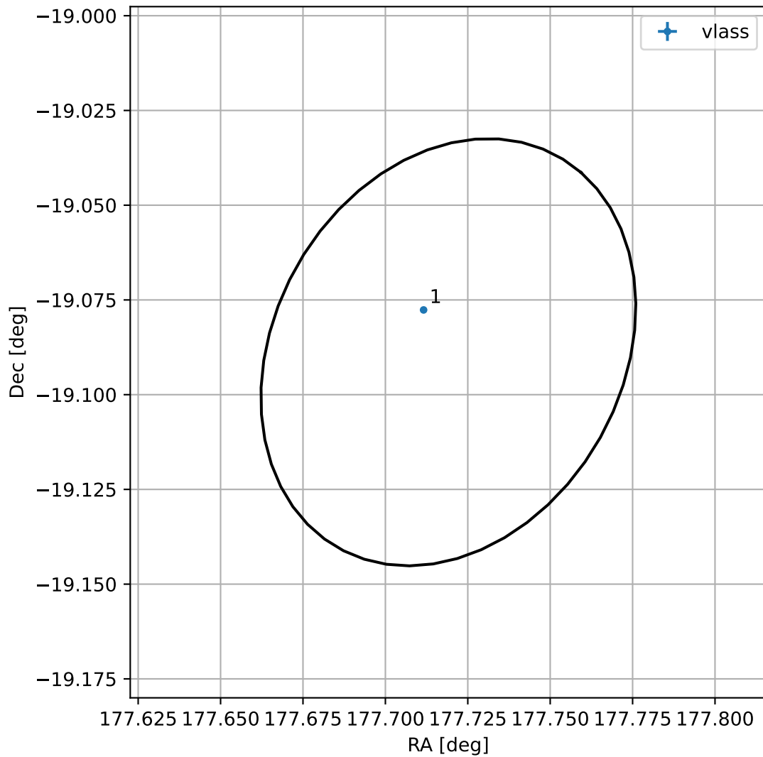
4FGL J1150.8-1905
