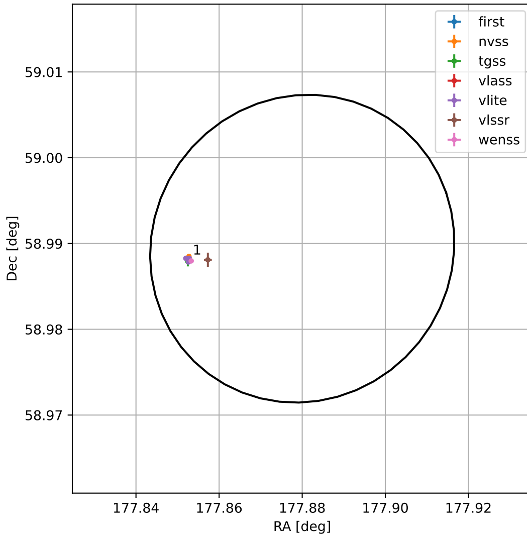
4FGL J1151.5+5859
