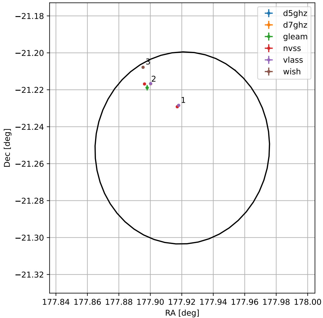
4FGL J1151.6-2115
