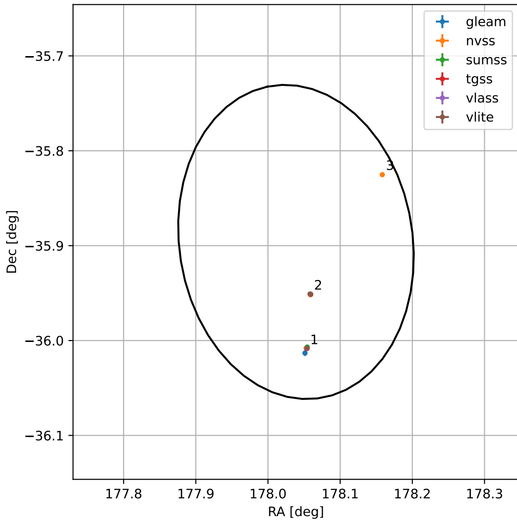
4FGL J1152.1-3553
