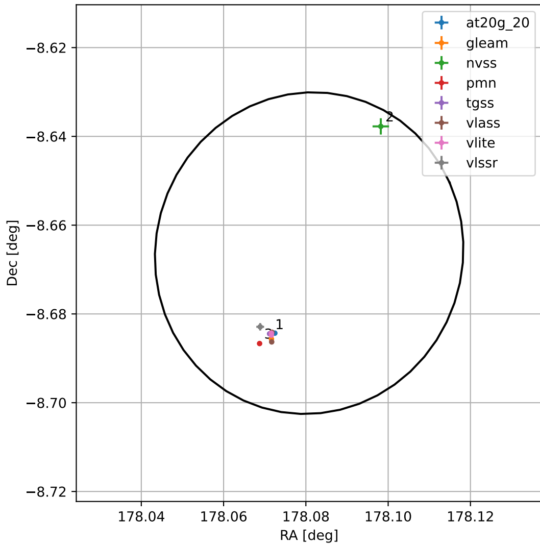
4FGL J1152.3-0839
