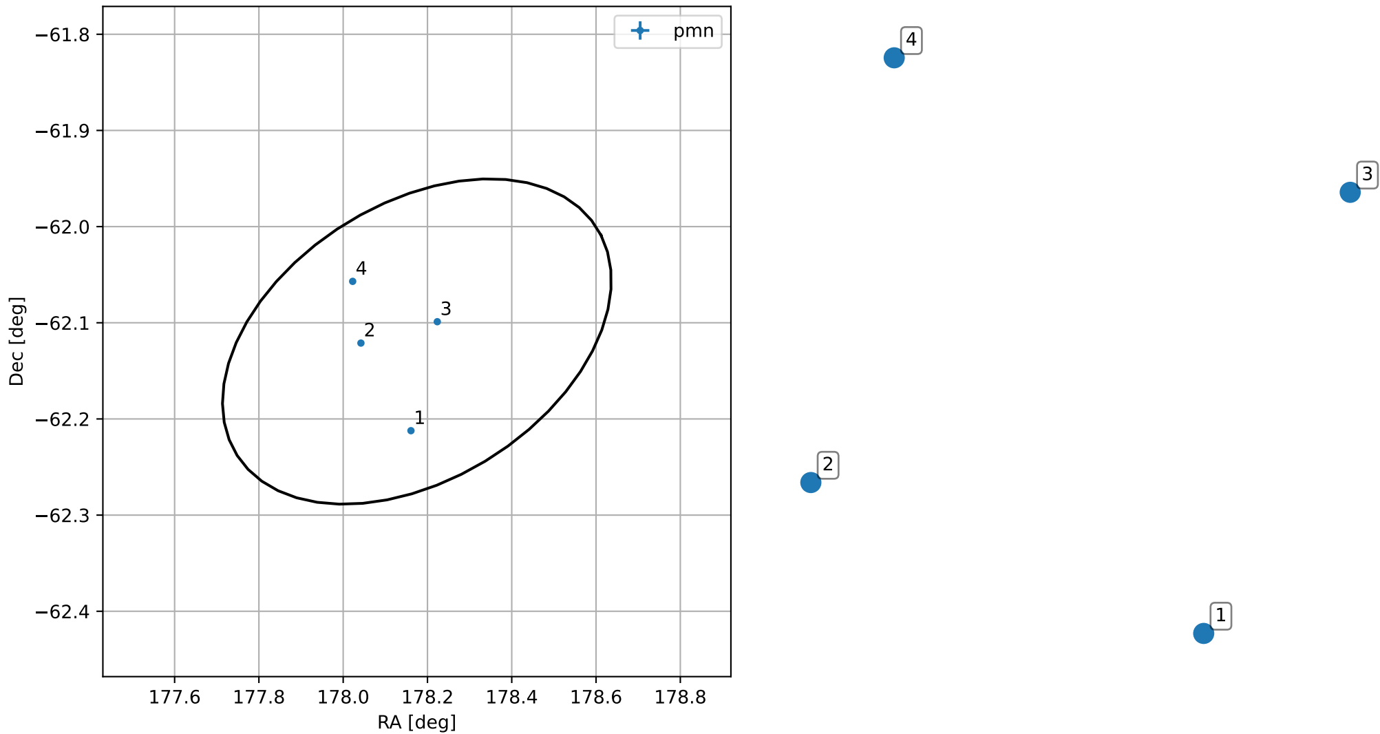
4FGL J1152.6-6207
