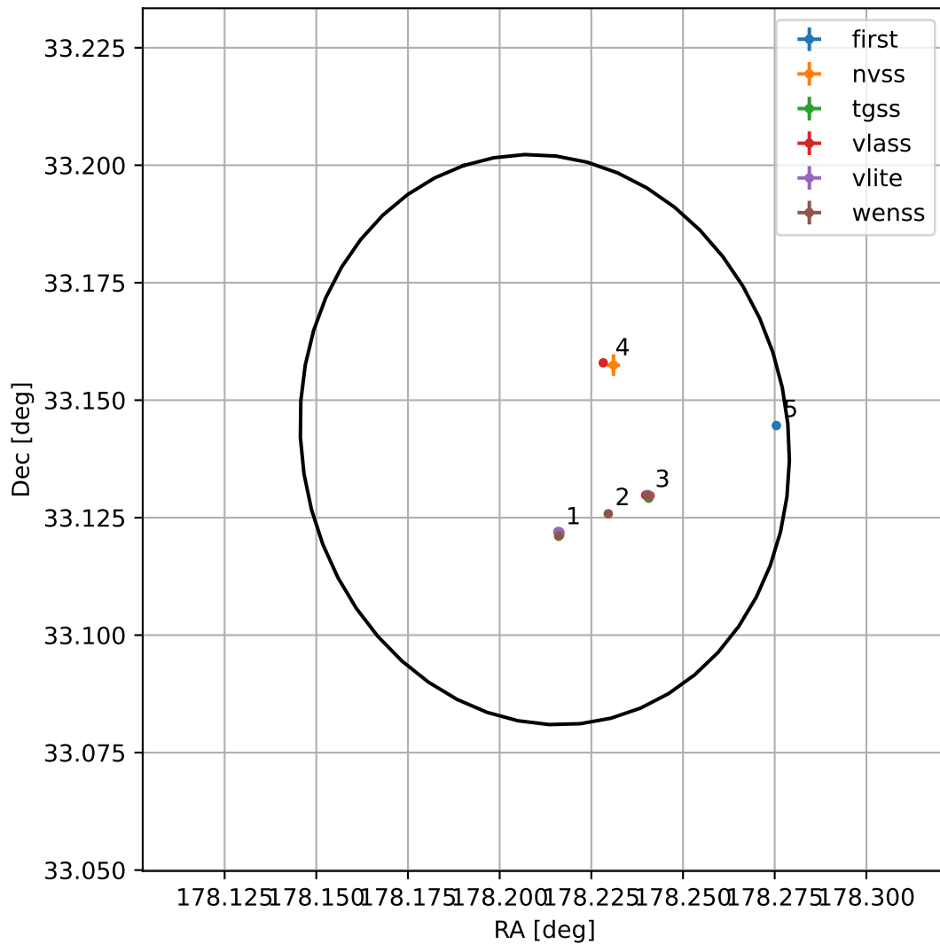
4FGL J1152.8+3308
