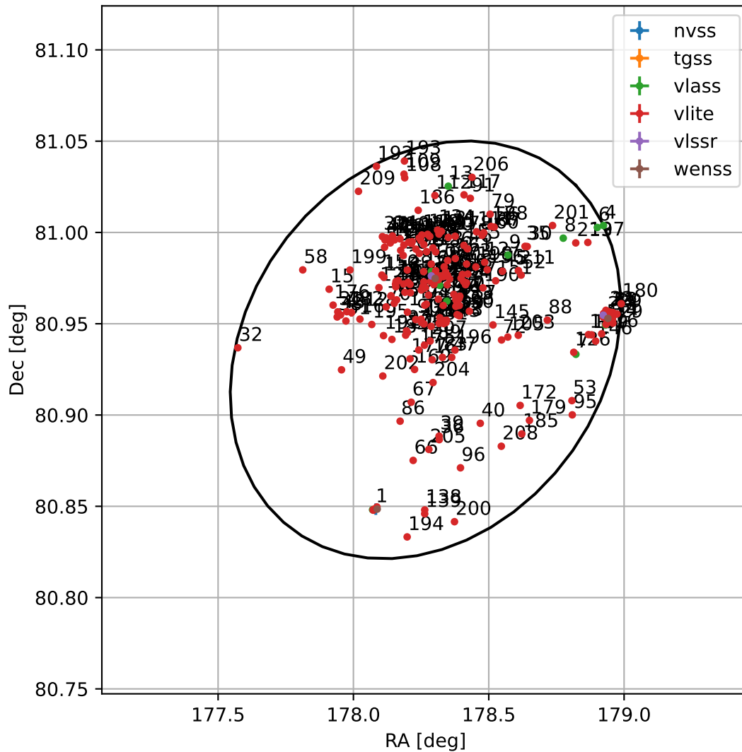
4FGL J1153.0+8056
