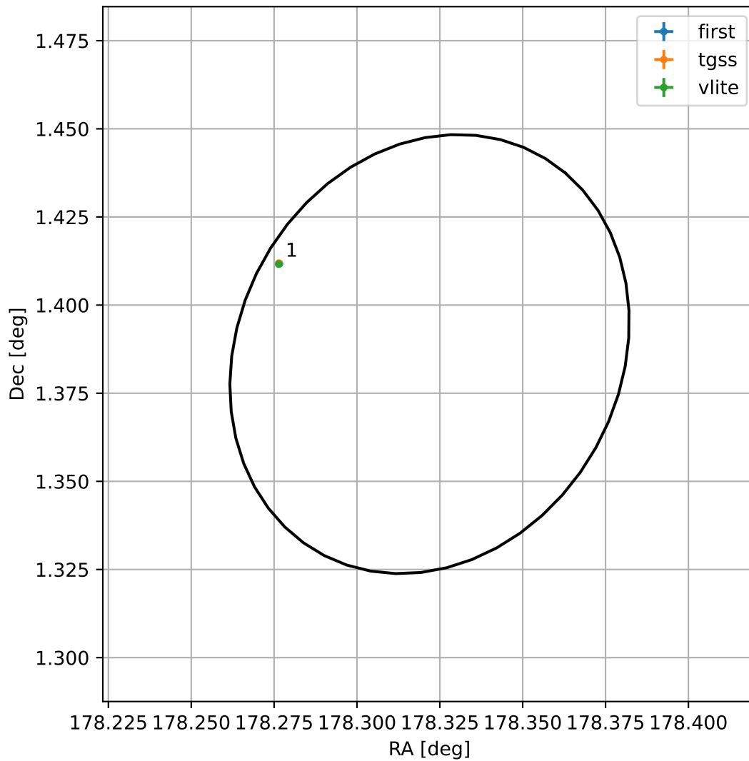
4FGL J1153.2+0123
