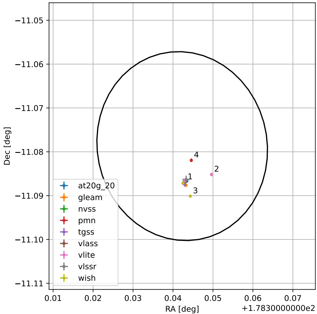
4FGL J1153.3-1104
