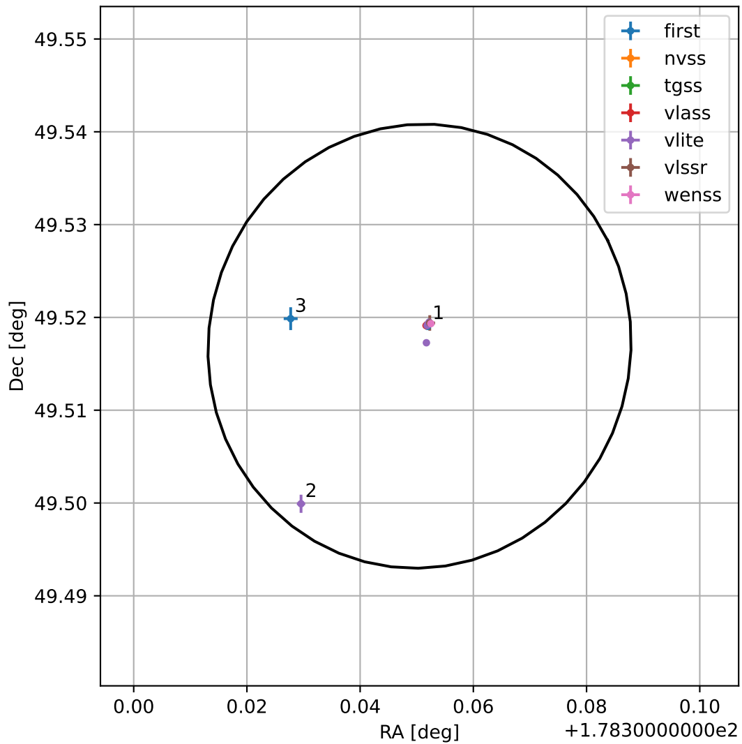
4FGL J1153.4+4931
