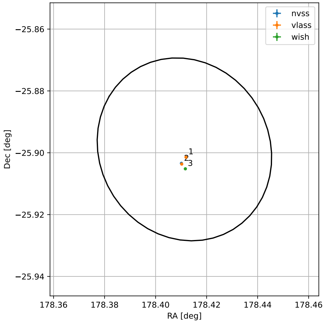
4FGL J1153.6-2553
