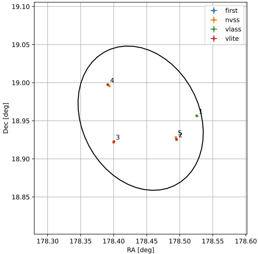
4FGL J1153.7+1857
