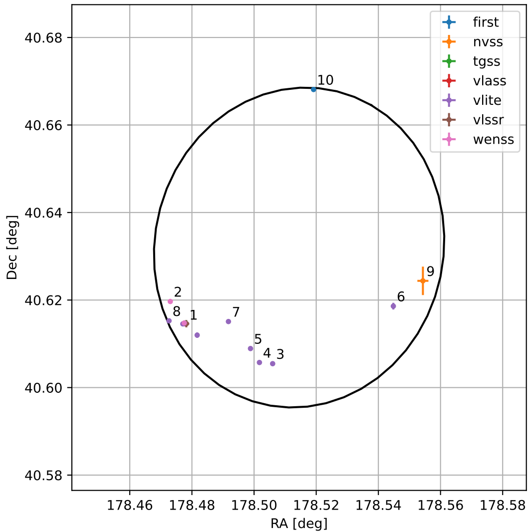
4FGL J1154.0+4037
