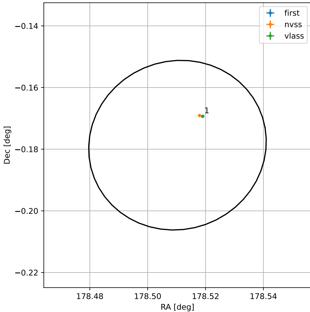
4FGL J1154.0-0010
