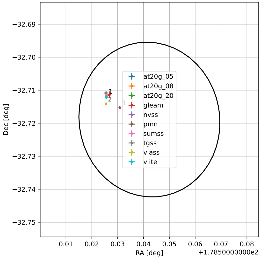
4FGL J1154.1-3243
