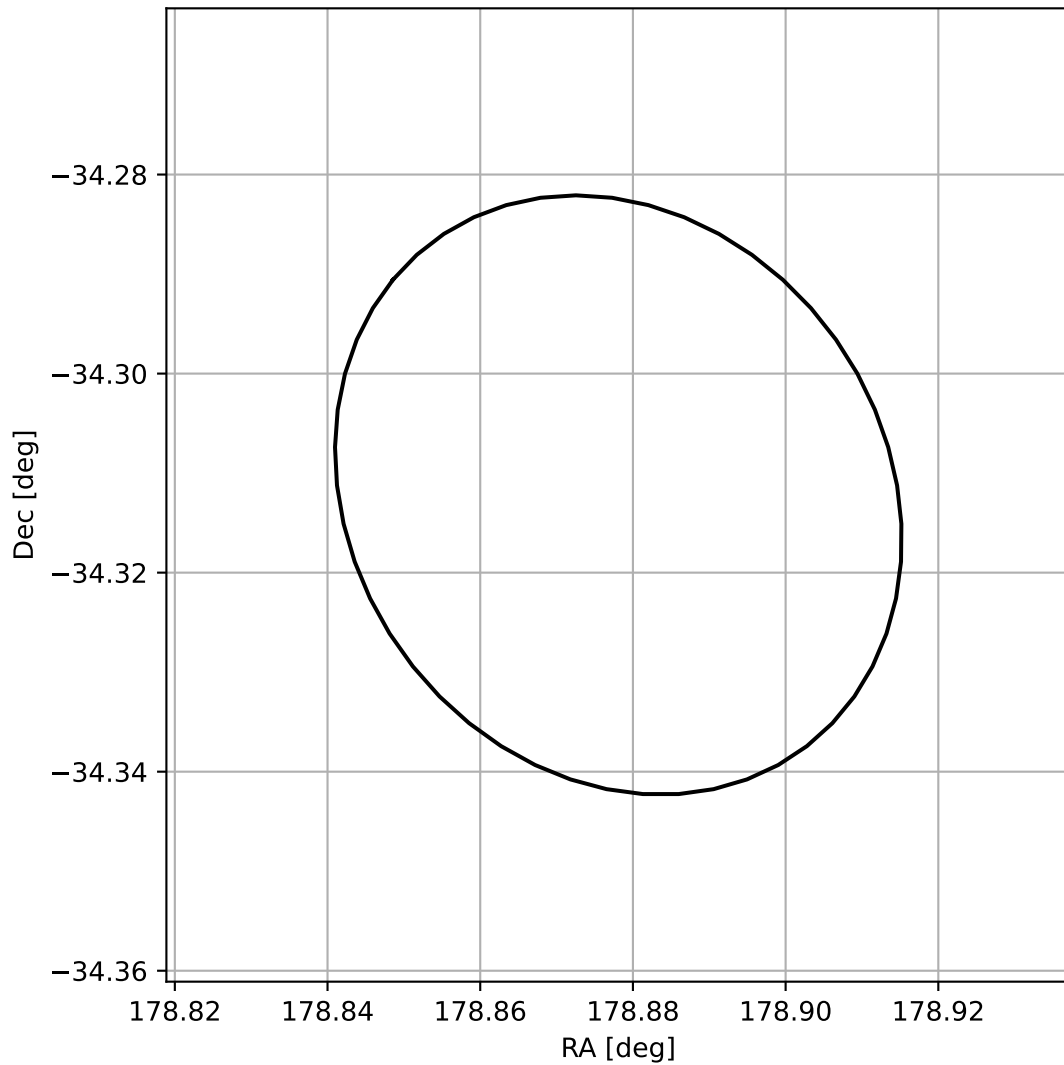
4FGL J1155.5-3418
