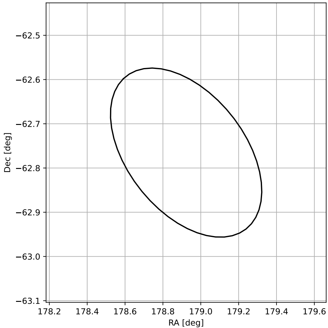
4FGL J1155.6-6245
