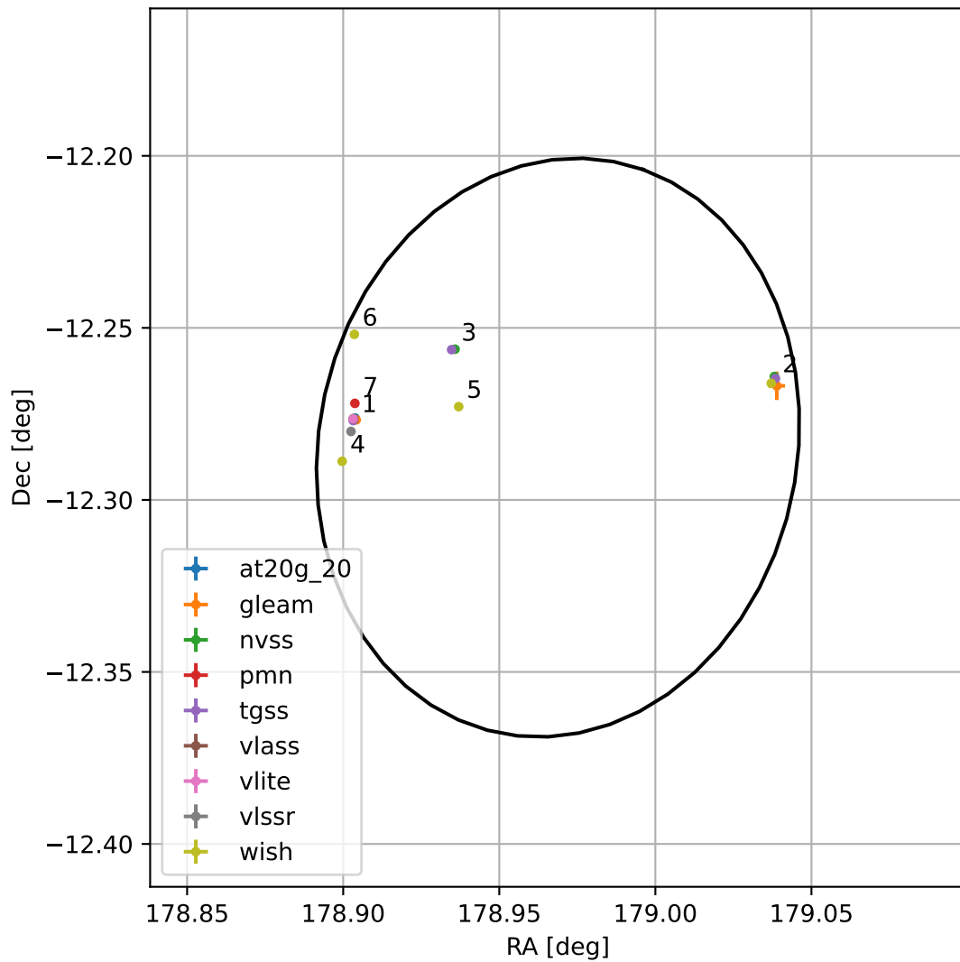
4FGL J1155.8-1217
