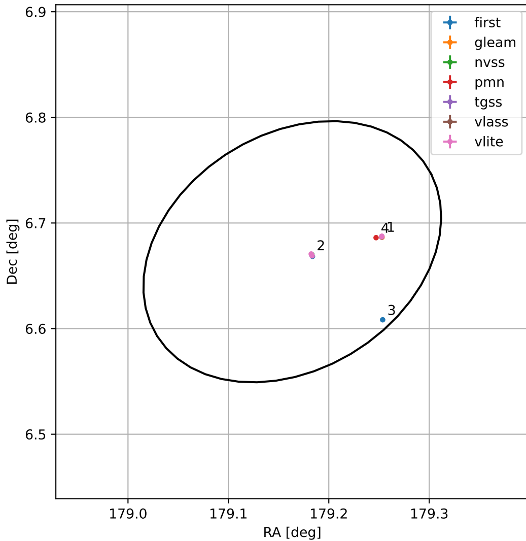
4FGL J1156.6+0640
