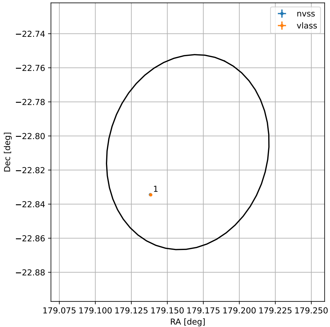
4FGL J1156.6-2248
