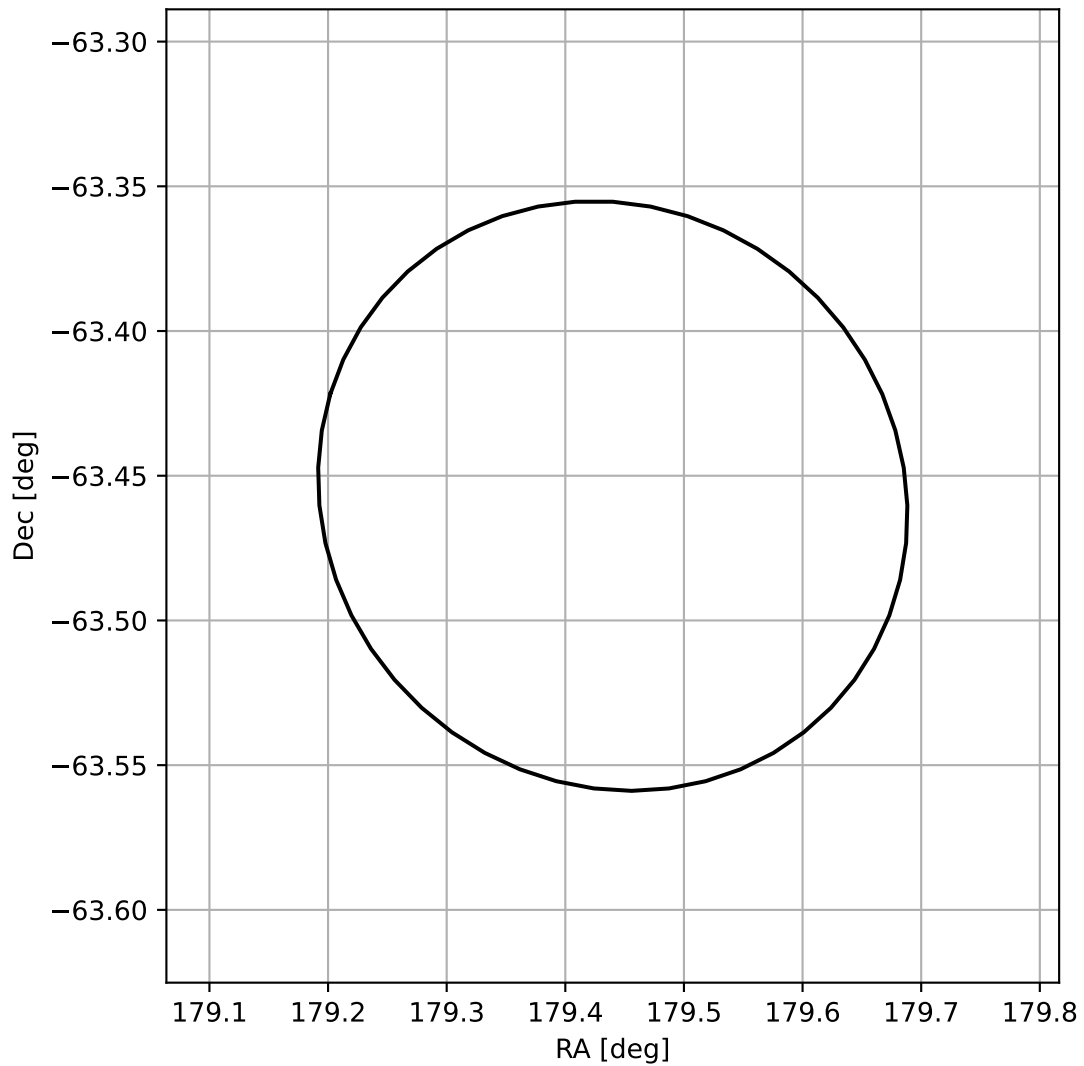
4FGL J1157.7-6327
