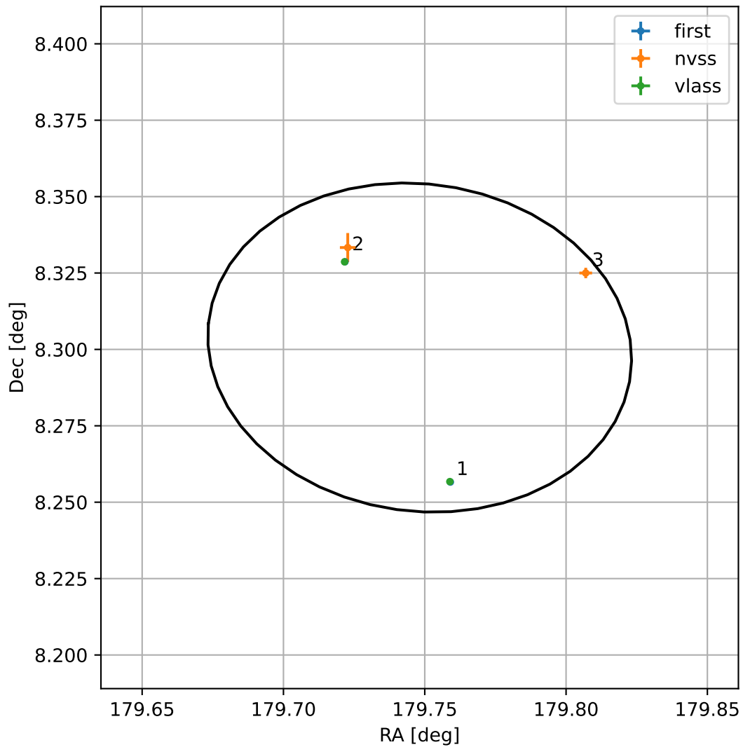
4FGL J1158.9+0818
