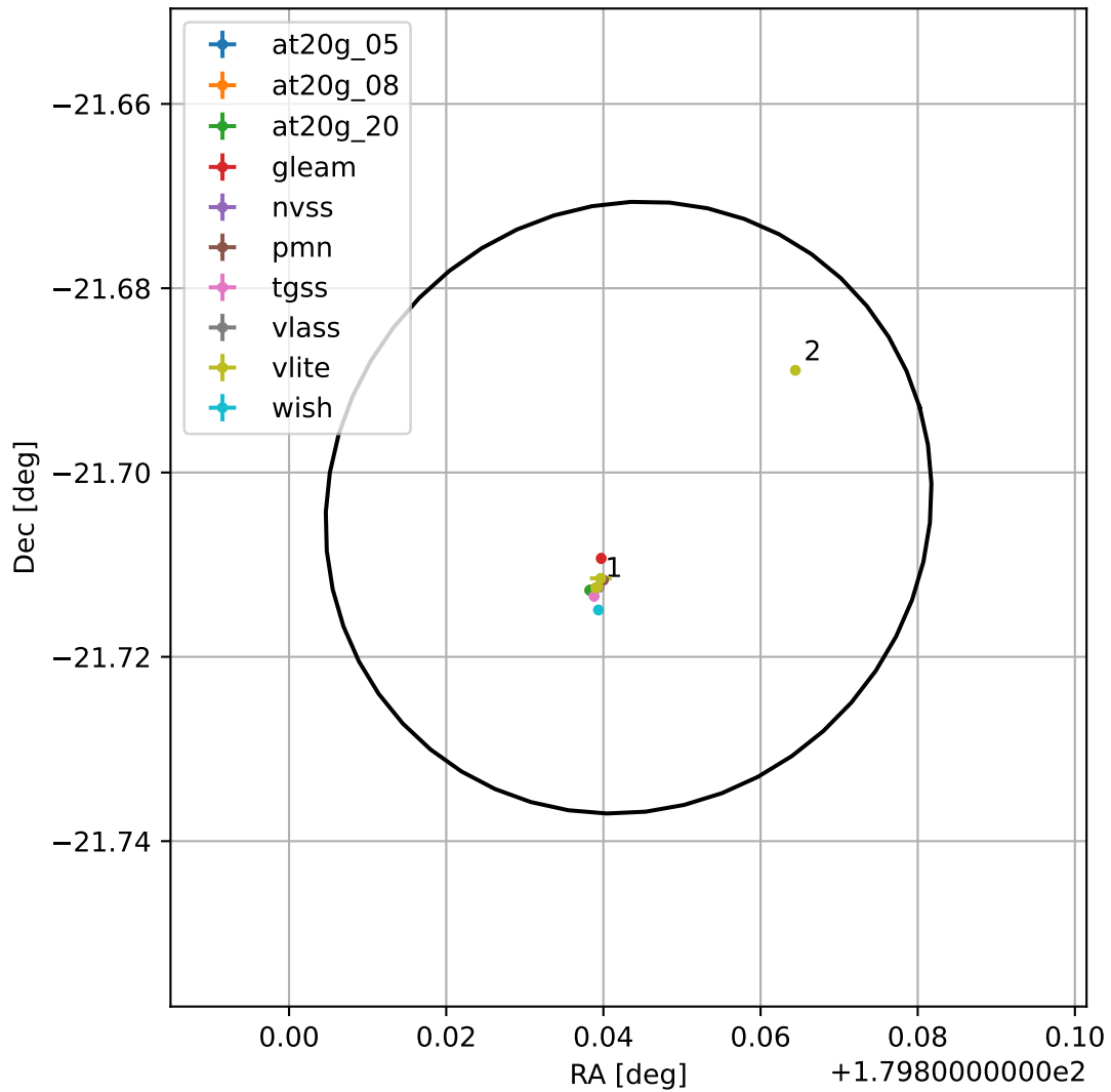
4FGL J1159.3-2142
