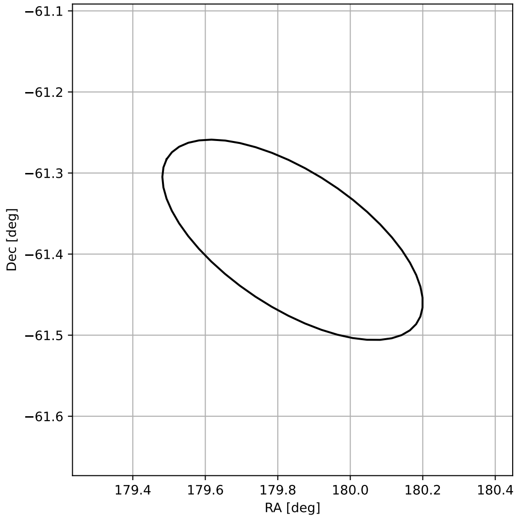
4FGL J1159.3-6122
