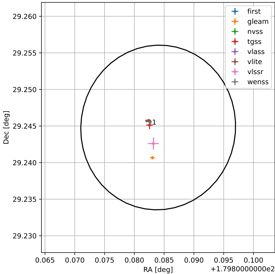
4FGL J1159.5+2914
