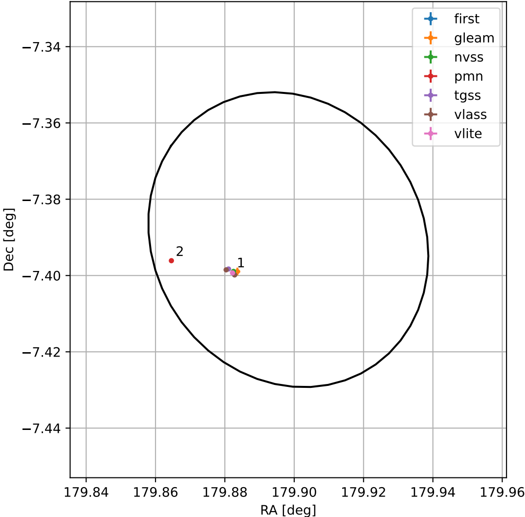
4FGL J1159.5-0723
