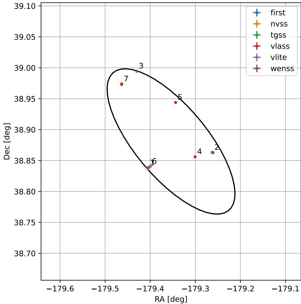
4FGL J1202.5+3852
