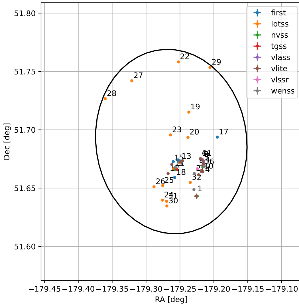
4FGL J1202.9+5141
