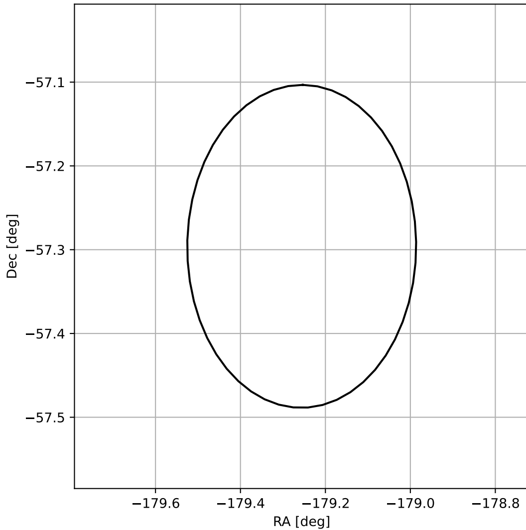
4FGL J1202.9-5717
