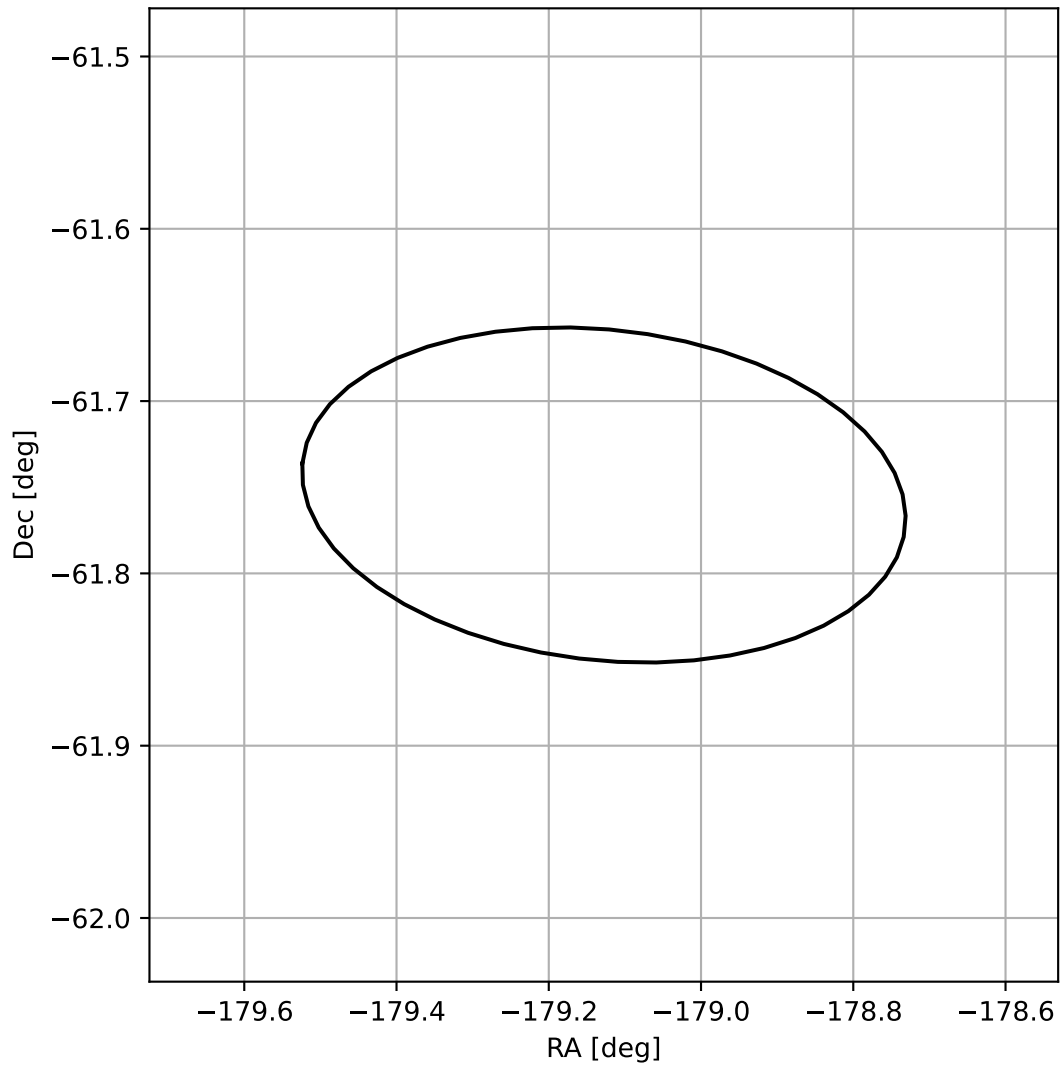
4FGL J1203.4-6145
