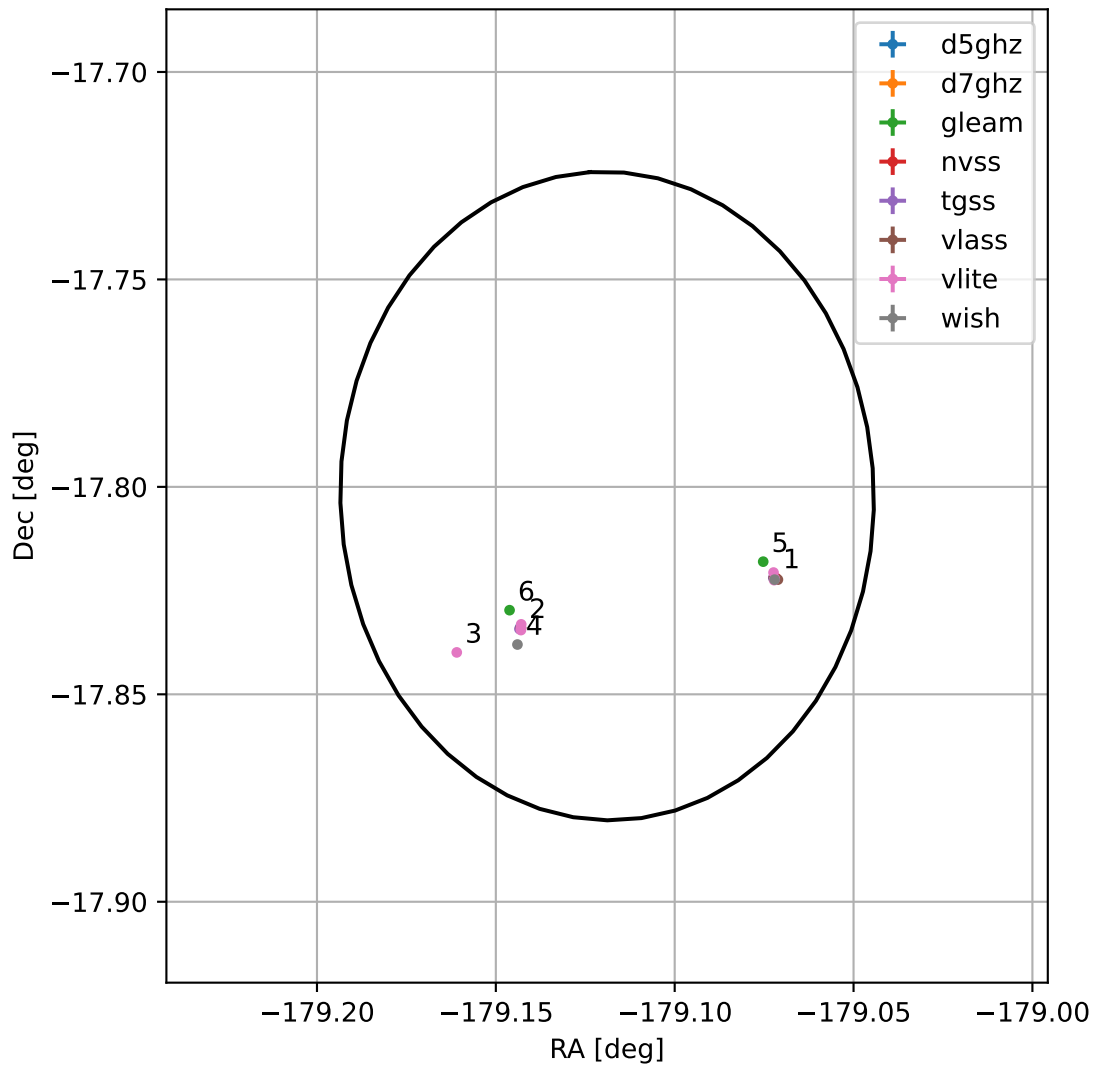
4FGL J1203.5-1748
