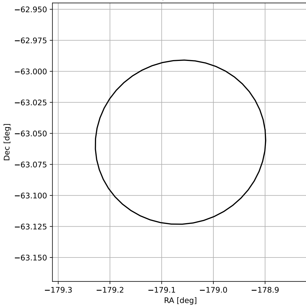
4FGL J1203.7-6303
