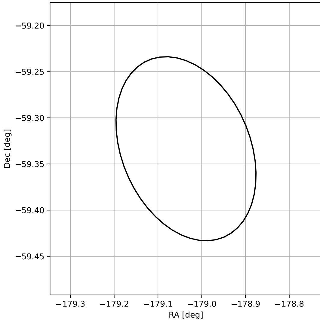
4FGL J1203.8-5920
