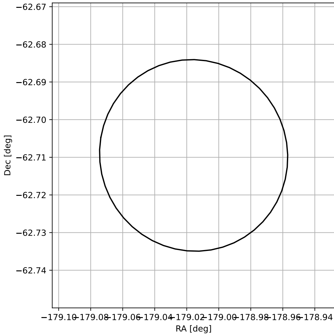
4FGL J1203.9-6242
