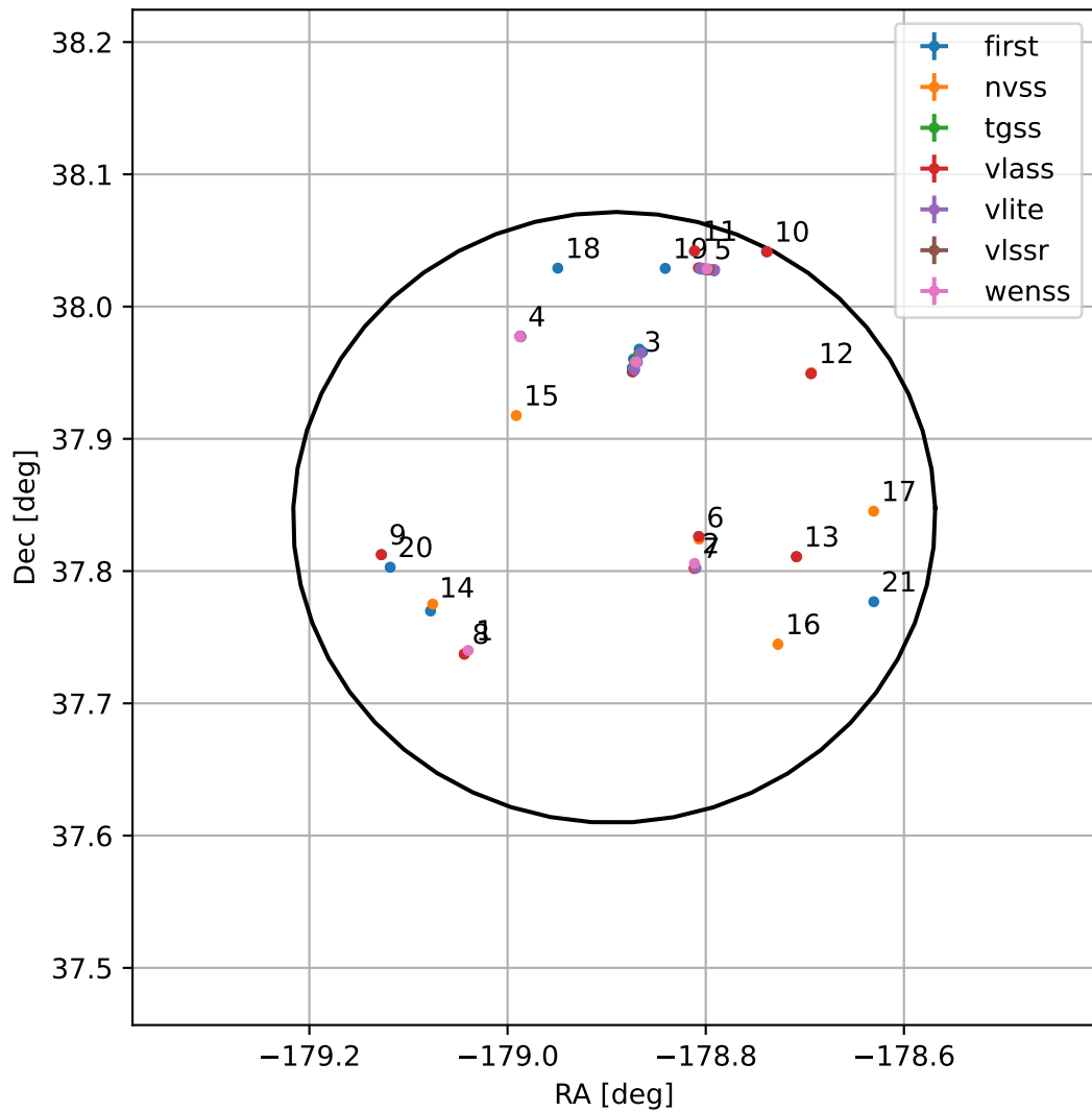
4FGL J1204.4+3750
