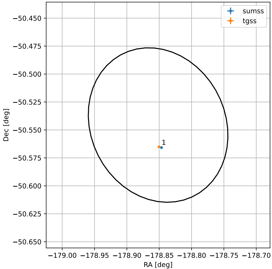
4FGL J1204.5-5032
