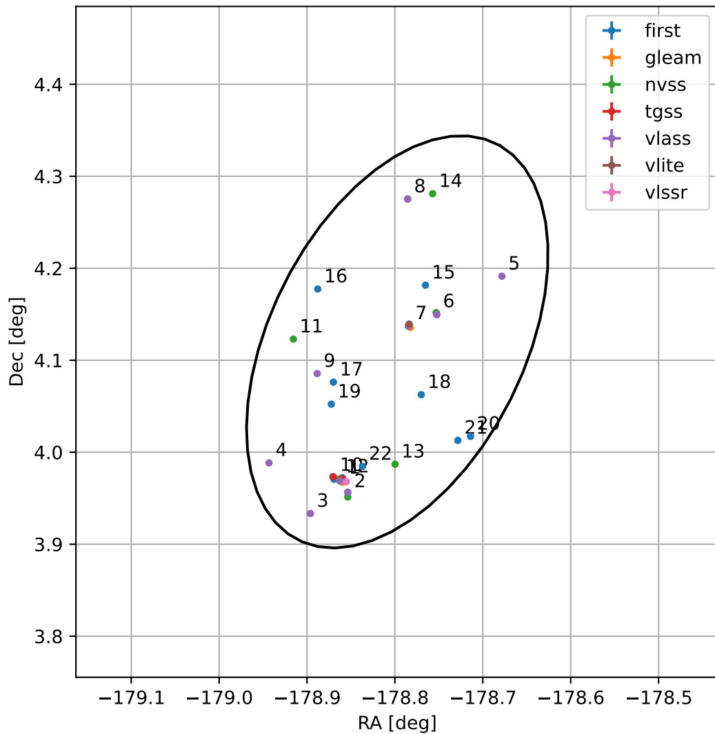
4FGL J1204.8+0407
